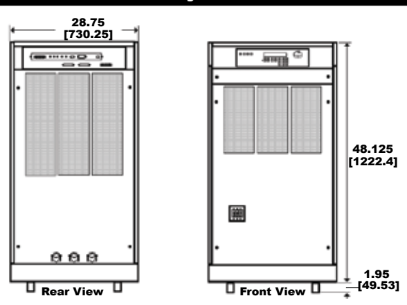
MX30/MX45 Dimensions - single chassis
