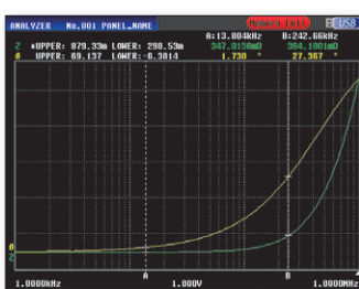
Frequency sweep measurement Z-θ measurement screen
