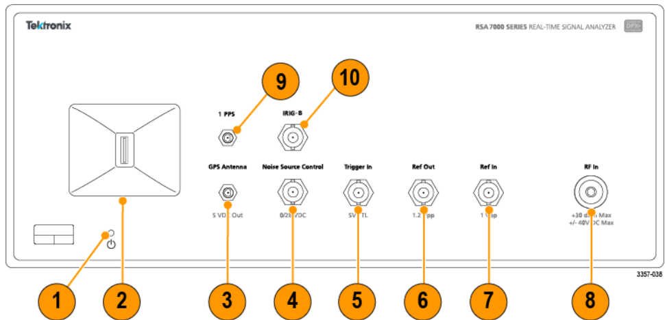
Figure 1: RSA7100 with Option GPS includes the IRIG-B and 1 PPS connectors
