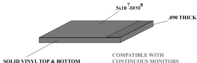
BOTRON SOLID VINYL MAT Meets ANSI/ESD S20.20 & EIA-625
